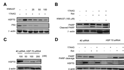
Fig. 4 Suppression of Hsp70 blocked the neuroprotection of 17-AAG. Cells were treated with KNK437, an inhibitor of Hsp 70, at various concentrations 1 h before 17-AAG treatment (A) and the effect of KNK437 on the inhibition of Hsp70 was evaluated by immunoblotting assay (A). Cells were pretreated with 17-AAG with or without KNK437 followed by adding rotenone for another 24 h and the apoptosis was assessed by detection the protein levels of cleaved PARP by immunoblotting assay (B). SH-SY5Y cells were transfected with Hsp70 siRNA at various concentrations for 72 h. Transfection of cells with silencer™ negative control #3 siRNA was used as a sham control (C). Protein levels of Hsp70 were measured by immunoblotting assay with anti-Hsp70 antibody. Cells with negative control #3 siRNA or Atp5 siRNA transfection were pretreated with 17-AAG for 24 h followed by addition of rotenone for another 24 h (D). The protein levels of cleaved PARP and Hsp70 were measured by immunoblotting assay. \beta -actin was used as an equal loading of proteins.
