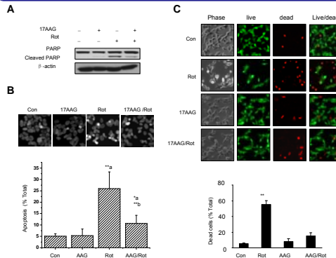
Fig.1 Neuroprotection of 17-AAG on rotenone-induced apoptosis in SH-SY5Y cells. The SH-SY5Y cells were pretreated with 17-AAG for 24h followed by addition of rotenone (10 \mu M) for another 24 h. Apoptosis was assessed by detection the protein levels of cleaved PARP by immunoblotting assay (A). Apoptotic cells were quantified by staining the nuclear with Hoechst 3334 (B, upper) and quantification of apoptosis were expressed as percentage of the total, and the values were the mean \pm SD (B, lower). Data were analyzed by one-way analysis of variance (ANOVA). * p < 0.01; ** p < 0.05 as compared with vehicle treated control (A), Rot group (B). (Con = control; Rot = rotenone). After specific treatment, live and dead cells were assayed by cell live/dead assay kit and determined under fluorescent microscopy (C, upper). The green fluorescence, generated by calcein AM, indicates live cells, and the red fluorescence, generated by ethidium homodimer-1, indicated dead cells. The number of dead cells was counted and value was expressed as percentage of total cells. Data were expressed as the means \pm SD (C, lower). ** P < 0.01 as compared to control.
