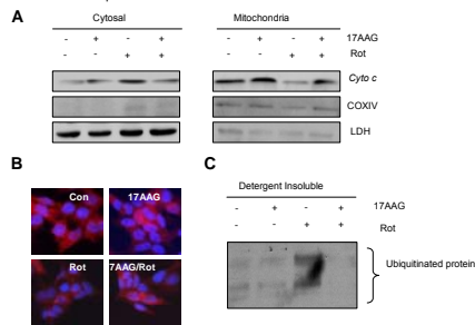
Fig.2 17-AAG attenuated rotenone-induced dysfunction of mitochondria and enhanced degradation of ubiquitinated proteins. The effect of 17-AAG on the release of cytochrome c was evaluated by immunoblotting assay with anti-cytochrome c antibody in both mitochondrial and cytosolic fractions (A). Mitotracker Red CMXRos at a final concentration of 500 nM was used to visualize the mitochondrial transmembrane potential (red, B). Blue indicates DAPI nuclear staining (B). The levels of ubiquitinated proteins from detergent-insoluble fractions of cells were detected by immunoblotting assay with anti-ubiquitin antibody (C).
